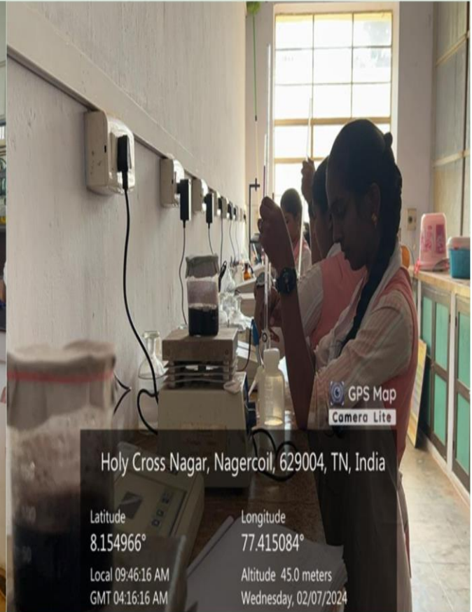
Conductometric Titrations
